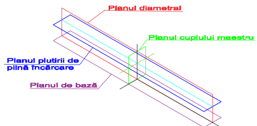
Figura 1-1.a. Planurile principale ale corpului navei [2], [3], [4], [5], [6], [7], [8], [9], [11], [12], [13], [14], [15], [16], [17], [18], [19], [20], [21], [22],[25], [29], [30], [32], [33], [34], [35], [36], [37], [38], [39].
